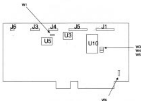
Figure 1. Jumper Locations
