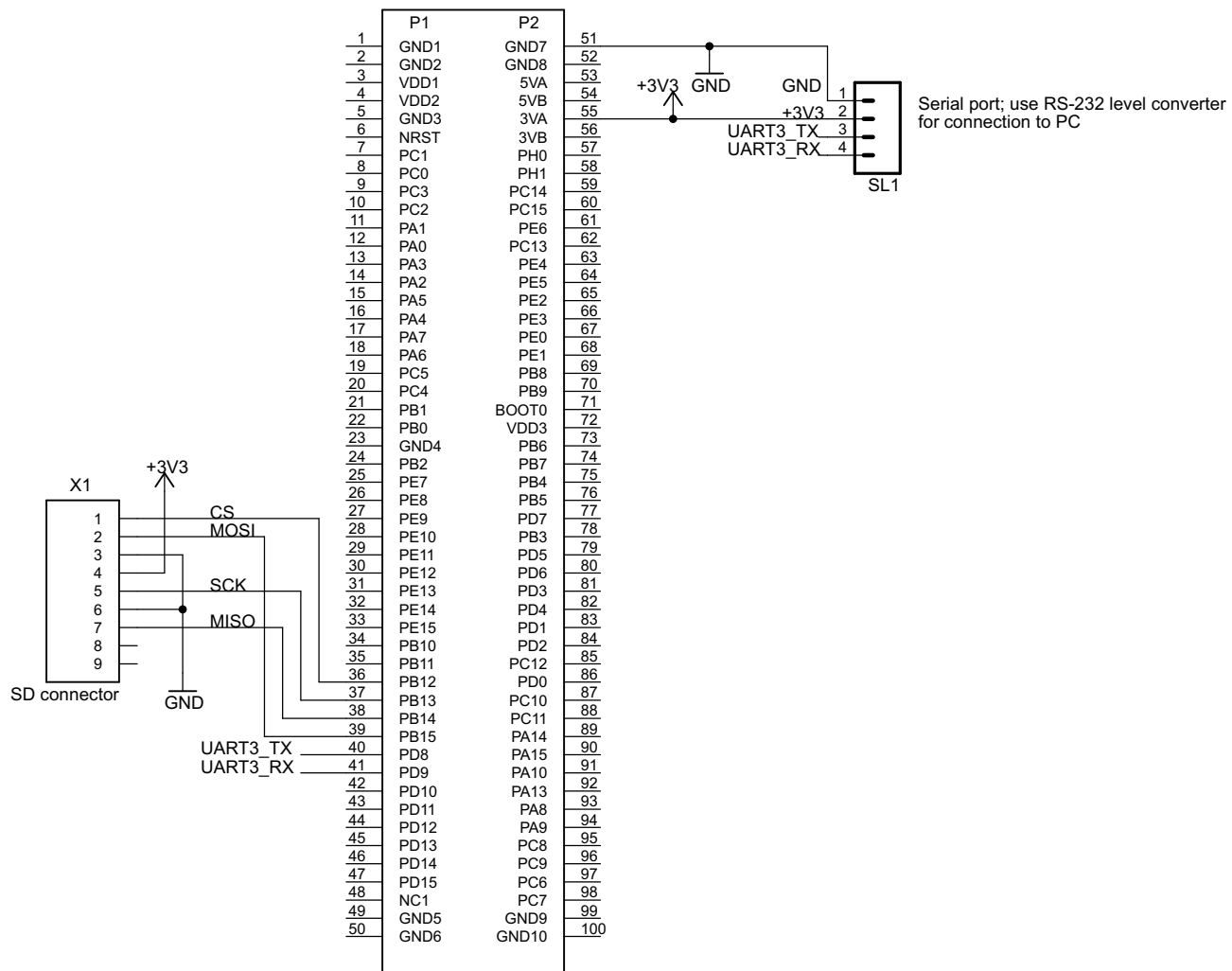
STMicro STM32F4 Discovery board
